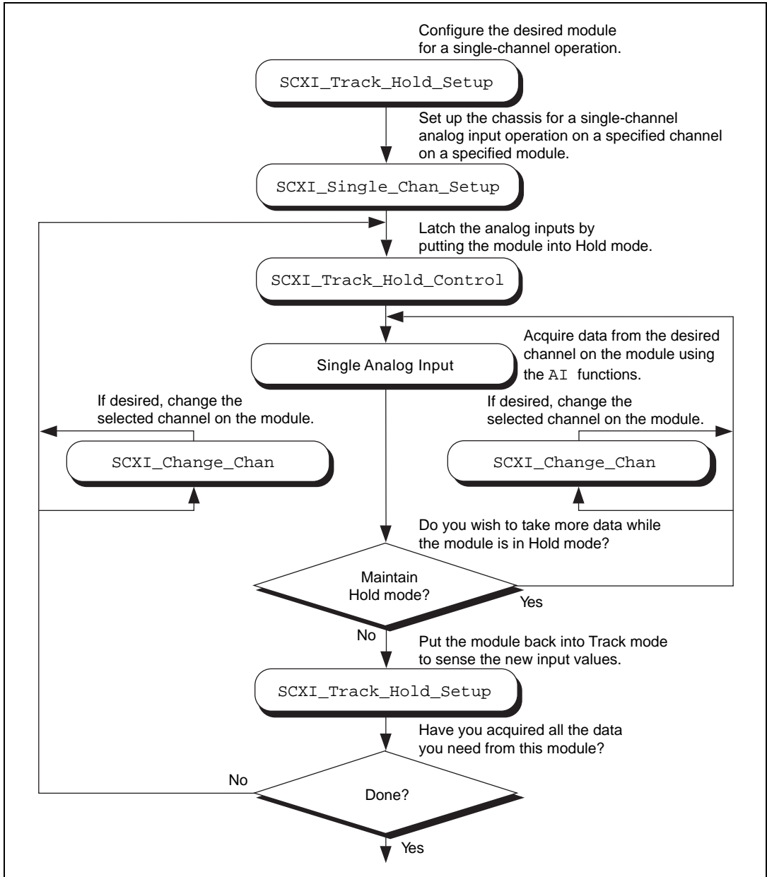
Figure 3-42. Single-Channel or Software-Scanning Operation Using a Track-and-Hold Module in Multiplexed Mode
