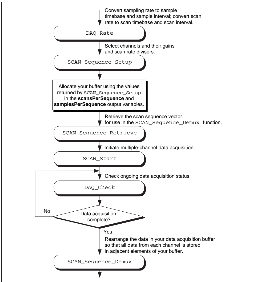
Figure 3-11. Multirate Scanning
